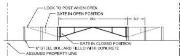
1 ELEVATION OF PROPOSED GATE
